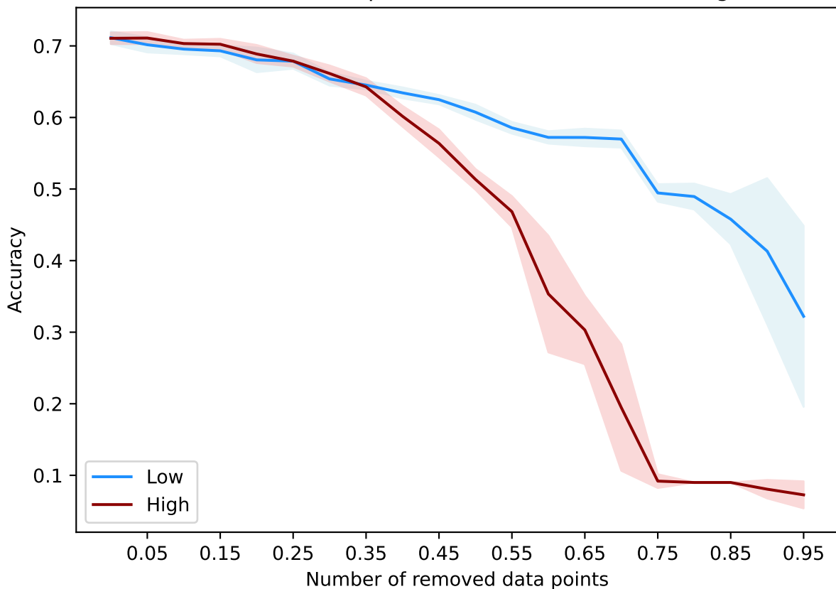
DataOob(1000, epochs=15) - cifar10-embeddings
